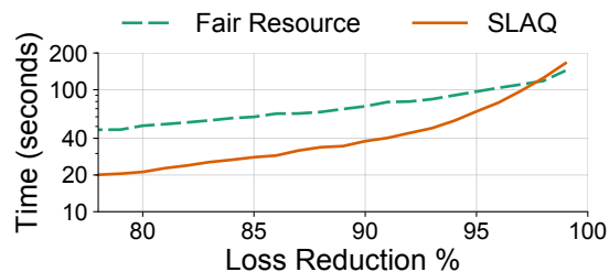
(b) Time to achieve loss reduction percentage.
