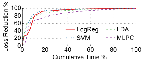
Figure 1: Cumulative time to achieve different percentages of loss reduction with four jobs: Logistic Regression (LogReg), Support Vector Machine (SVM), Latent Dirichlet Allocation (LDA) and Multi-Layer Perceptron Classifier (MLPC). Job convergence is defined to be 1/10000 of initial loss reduction.
