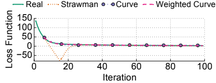
(a) Predicting loss values 10 iterations in advance.
