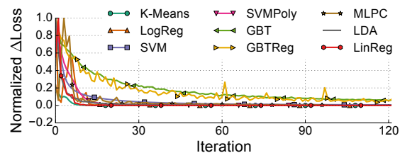
Figure 5: Normalized \Delta Loss for ML algorithms.
