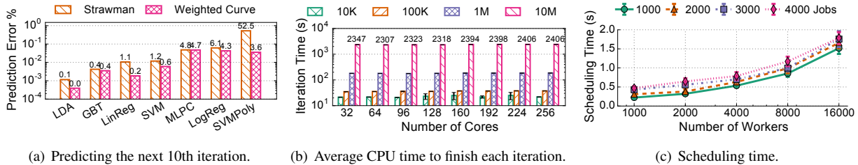
Figure 10: SLAQ loss / runtime prediction and overhead.
