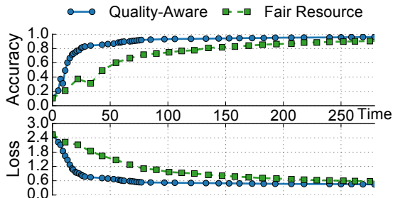
Figure 3: Accuracy (top) and loss function values (bottom) of a job with resources allocated by a quality-aware scheduler and a fair scheduler. Accuracy (percentage of correctly predicted data points) is evaluated on a testing dataset at the end of each training iteration. The more resources allocated to a job, the faster an iteration can be finished.
