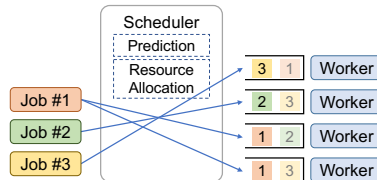
(b) Scheduler Architecture
