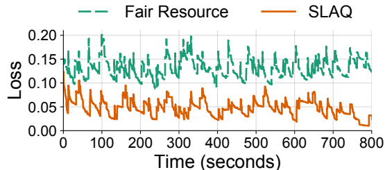
(a) Average of normalized loss values.
