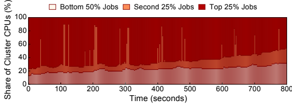
Figure 8: Resource allocation across jobs. At the beginning, jobs with the greatest 25% loss allocated vast majority of resources; towards the end, the difference in loss shrinks, the allocation is more spread out.
