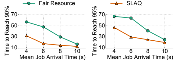
Figure 9: The performance difference between SLAQ and a fair resource scheduler is more significant under workloads with greater contention, e.g., jobs arriving with a mean arrival time of 4s compared to 10s.
