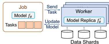
(a) Distributed ML Training
